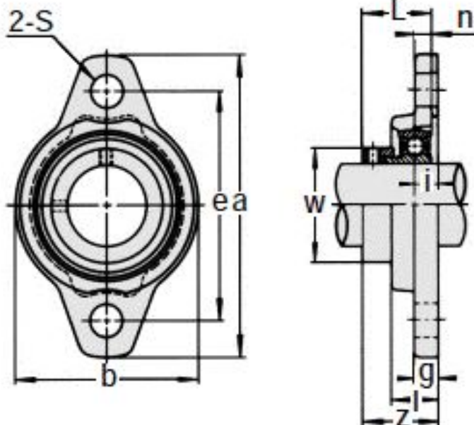
UFL Shape (Eccentric Collar System)
